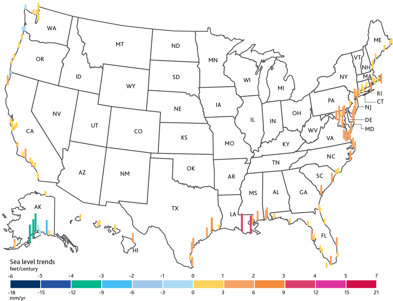
Exhibit 5 Sea levels have risen in coastal areas of the US
