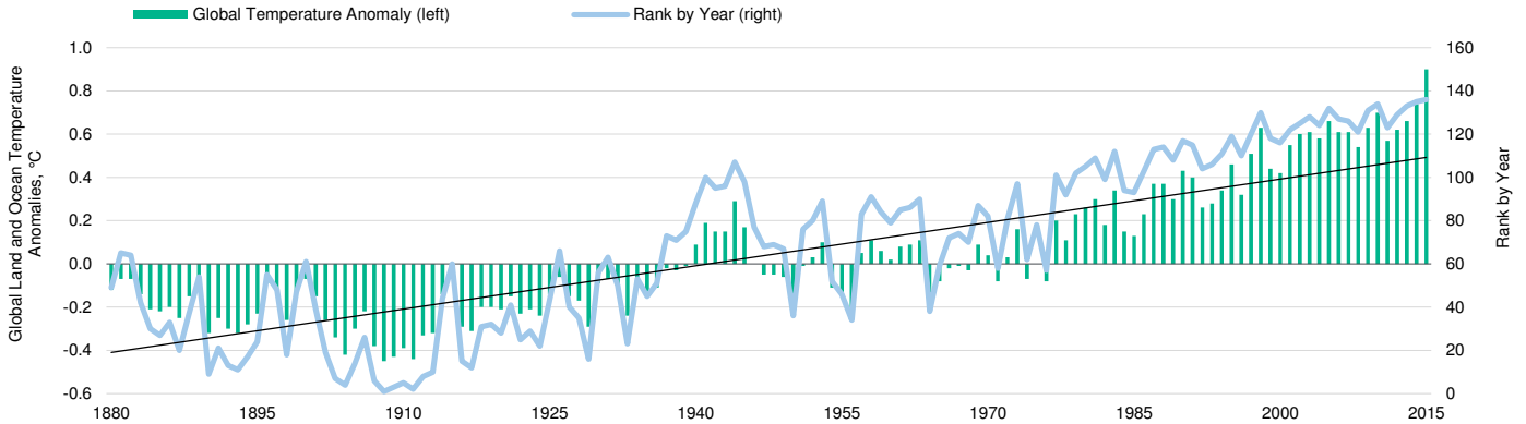
Exhibit 3 Global average temperatures continue to rise Global land and ocean temperature anomalies, 1880-2015
