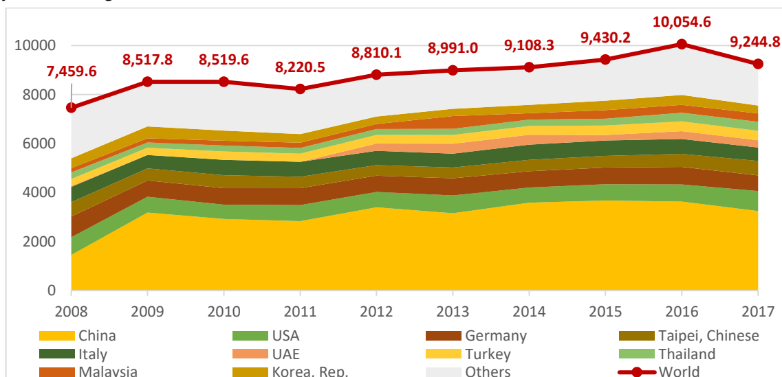
Figure 4.79. World refined copper import dynamics in 2008–2017, kt Source: ITC
