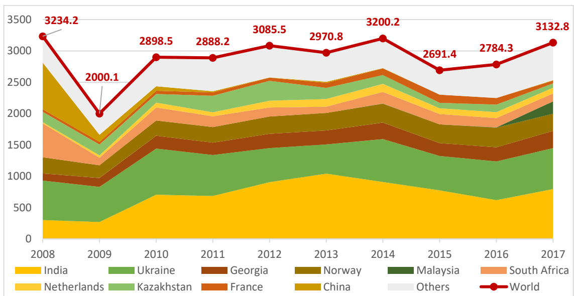
Figure 4.100. World silico-manganese export dynamics in 2008–2017, kt
