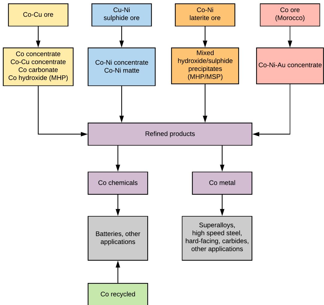
Figure 4.5. Cobalt value chain
