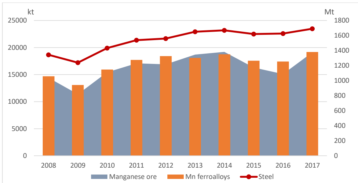
Figure 4.37. Dynamics of manganese ore production in terms of metal and manganese ferro-alloys (left scale) and steel (right scale) in 2008–2017 Sources: USGS, BGS, IMnI
