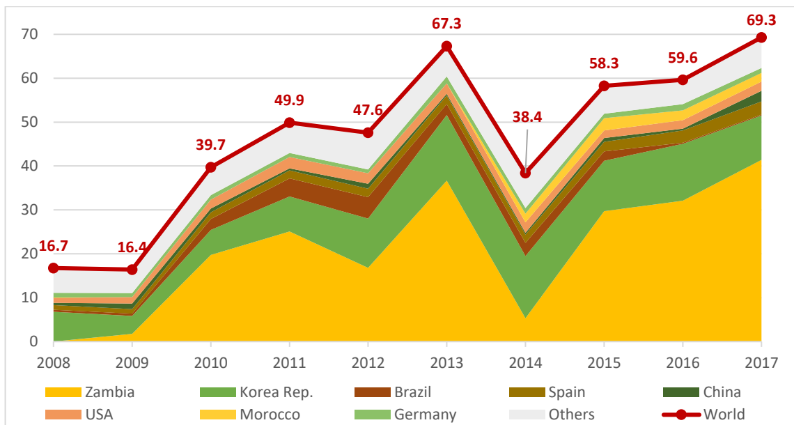
Figure 4.95. World cobalt oxides and hydroxides import dynamics in 2008–2017, kt Source: ITC
