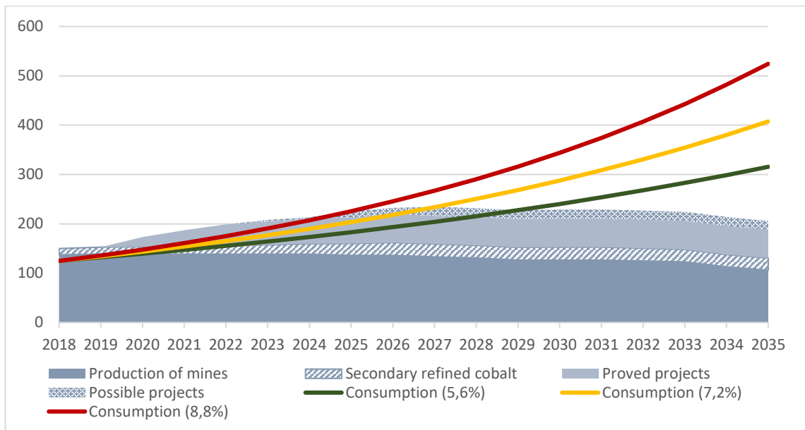
Figure 4.31. Cobalt land-based production and consumption forecast in 2018–2035, kt
