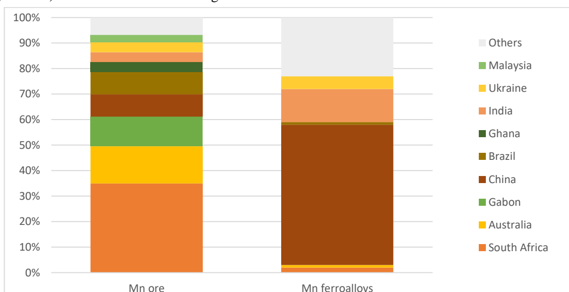
Figure 4.62. Distribution of production of manganese ore by content of manganese and ferro-alloys gross weight among major countries in 2017, % Source: IMnI
